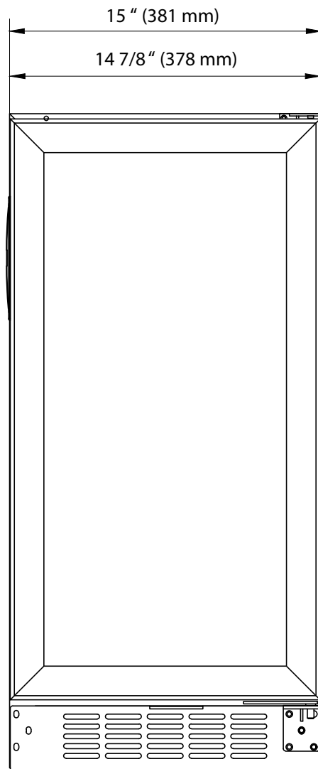
Front View
