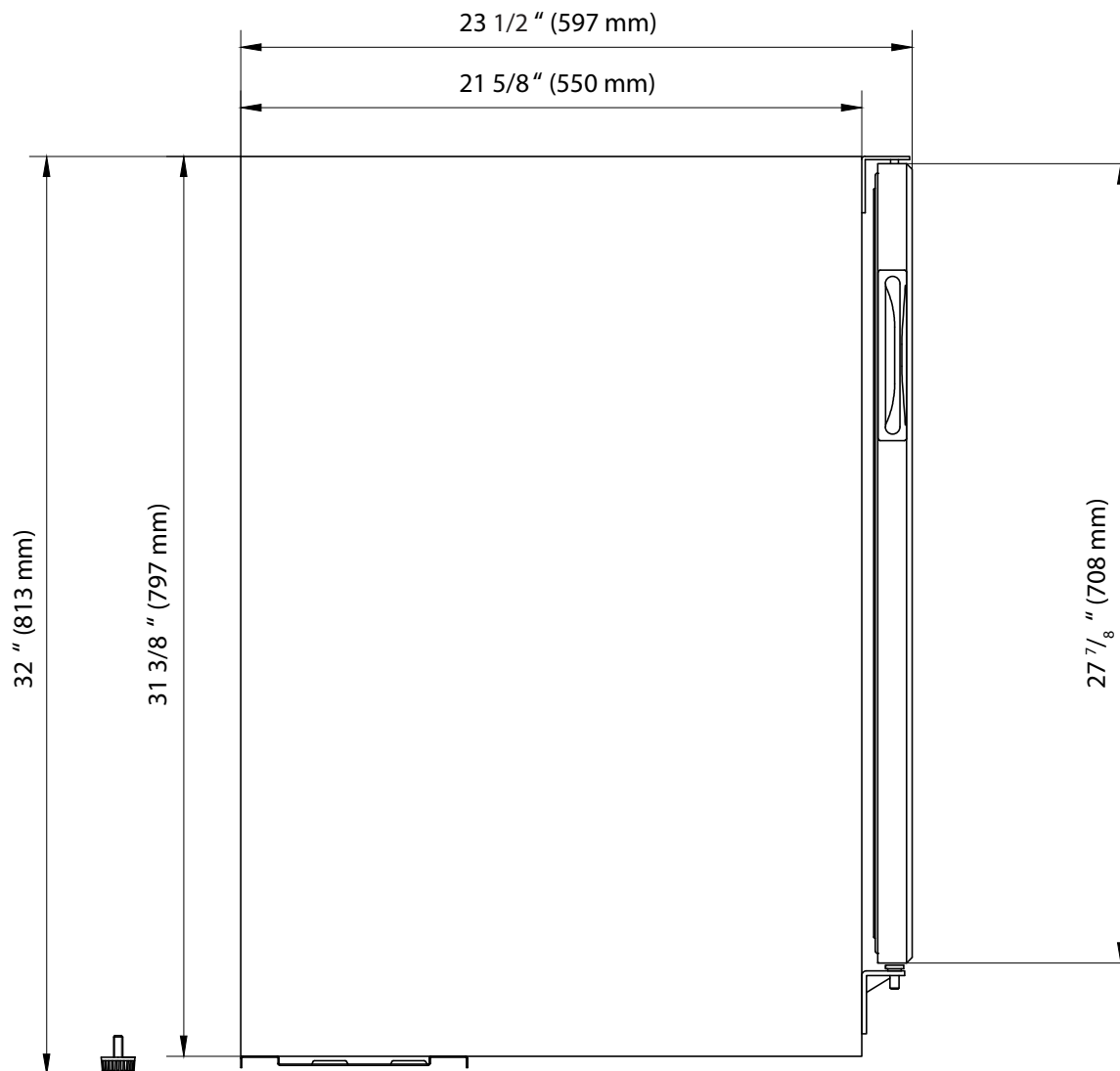
Side View
